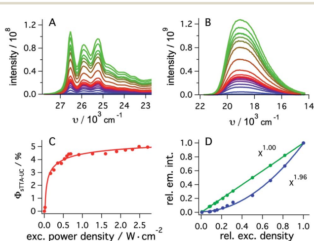
Fig. 4 (A) Upconverted {}^t\text{BuPy} fluorescence sensitized by \text{fac}[\text{Ir}(\text{ppy})_3] (30 \mu\text{M} ) in de-aerated DMF at 20 ^\circ\text{C} . Excitation occurred with a 447 nm cw-laser at various excitation densities in the presence of {}^t\text{BuPy} (5 mM). Excitation powers ranged from 2 mW to 338 mW. (B) Emission spectra of \text{fac}[\text{Ir}(\text{ppy})_3] recorded under identical conditions as for (A) but in the absence of {}^t\text{BuPy} . (C) Upconversion quantum yield ( \phi_{\text{sTTA-UC}} ) as a function of excitation power density as determined from eqn (1) and the data in (A) and (B), using a luminescence quantum yield ( \phi_{\text{ref}} ) of 0.88 for \text{fac}[\text{Ir}(\text{ppy})_3] . (D) Relative integrated intensities of upconverted {}^t\text{BuPy} (1 mM) fluorescence (blue circles) sensitized by \text{fac}[\text{Ir}(\text{ppy})_3] (10 \mu\text{M} ) upon excitation at 450 nm as a function of the relative excitation density. The solid blue line represents the best fit with a power function ( f(x) = a \times x^b + y ) to the experimental data, yielding b = 1.96 as indicated by the inset. The green circles result from an analogous experiment in which \text{fac}[\text{Ir}(\text{ppy})_3] was excited in the absence of {}^t\text{BuPy} under otherwise identical conditions, and the prompt luminescence emitted by \text{fac}[\text{Ir}(\text{ppy})_3] was monitored (Section 2.5.2 of the ESI†). In this case, a fit to the same power function (green solid line) yields an exponent of 1.00. Measurements in C occurred with the abovementioned cw-laser source, whilst measurements in D were performed using the excitation beam of the luminescence spectrometer.
