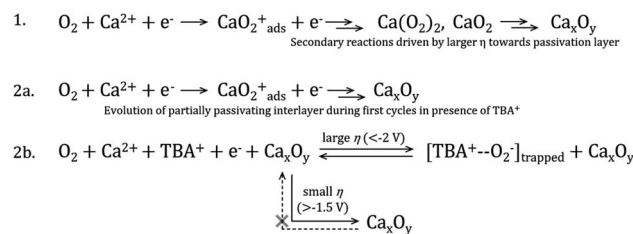
Scheme 1 Proposed ORR mechanism in DMSO electrolytes containing either (1) only Ca 2+ cations or (2) both TBA + and Ca 2+ . Line 2a represents the first few cycles at the pristine Au electrode where no quasi-reversible OER is observed, whereas line 2b illustrates the new trapped interfacial redox of the [TBA^+-O_2^-] species at the Ca x O y /Au interface under larger overpotentials ( \eta ). Voltages approximated from experimental work but specific critical limits will also depend on electrolyte composition and salt concentrations.
