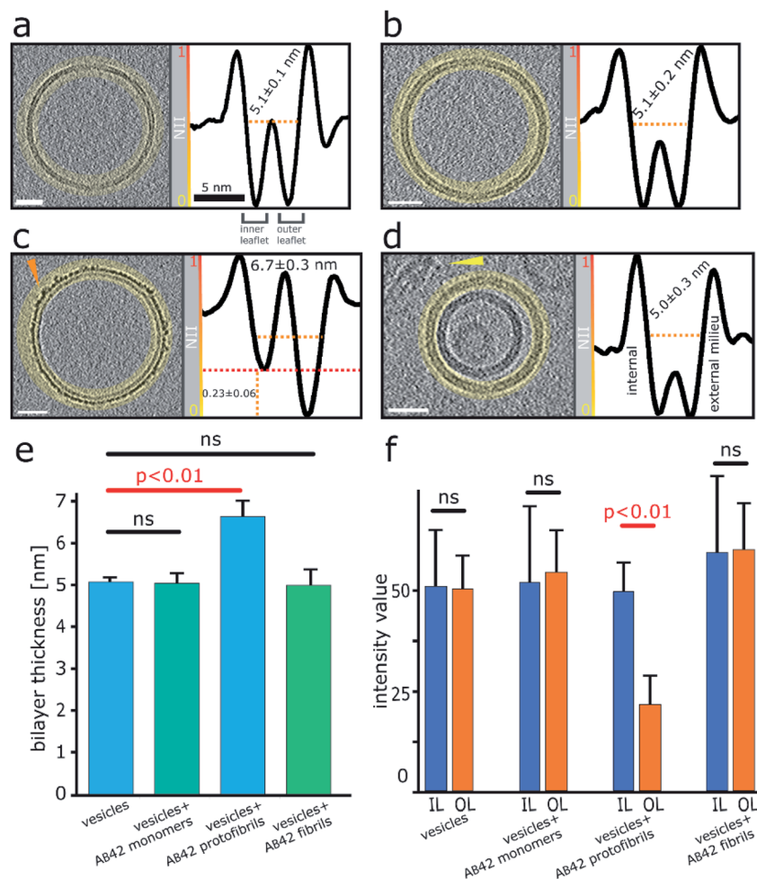
Fig. 3 Quantification of A \beta 42 insertion into outer-leaflet of lipid bilayers, measured by grey-scale intensity profile plots. (a) Liposome, no A \beta . (b) Monomeric A \beta . (c) Lag-phase A \beta oligomers/protofibrils. (d) A \beta fibrils. (a–d) Tomographic slices, 7.6 nm thick (left panels, scale bars: 25 nm) and the corresponding profile plots of normalized integrated intensities (NII) around the entire vesicle (highlighted in yellow and shown in the right panels). The minimal NII values correspond to the dark densities; indicating lipid membrane. The double dip intensities indicate the presence of the inner- and outer-membrane leaflet. A \beta free vesicles, A \beta monomer and A \beta fibril shows similar density for the inner and outer-leaflet. In contrast for A \beta oligomers the outer leaflet has significant additional density (red dotted line). (e) The thickness of the membrane, along with standard deviations, is also indicated for all four conditions. A bar-chart summarizes the thickness of the membrane measured at NII = 0.5, for 5 vesicles for each condition (>1000 nm of membrane for each condition), corresponding values are displayed on relevant panels (a–d). Only A \beta oligomer/protofibrils carpet the membrane and so appear significantly thicker by an average of 1.6 nm (ANOVA analysis). (f) The absolute intensity values around vesicles perimeters were compared for the inner leaflet (IL) and outer leaflets (OL). Only bilayer with A \beta 42 oligomers show a significant increase in density for the out-leaflet. Arrowheads point to an A \beta 42 protofibril in panel (c) and A \beta 42 fibril bundle in panel (d). See Movie M1† for Z-stacked slices through the vesicle shown in panel (c).
