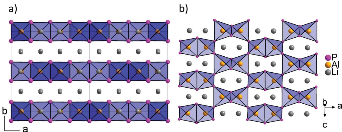
Fig. 3 Structural details of Li_3AlP_2 : (a) layers of ^2_\infty [AlP_2^{3-}] poly-anions are separated by lithium ions. (b) Top view of one ^2_\infty [AlP_2^{3-}] layer of dimers of two edge-sharing AlP_4 tetrahedra that are interconnected by vertex-sharing. Unfilled voids within the layer are filled with additional Li ions. AlP_4 tetrahedra are shown as blue polyhedra. Al, P and Li atoms are drawn in orange, purple and grey, respectively.
