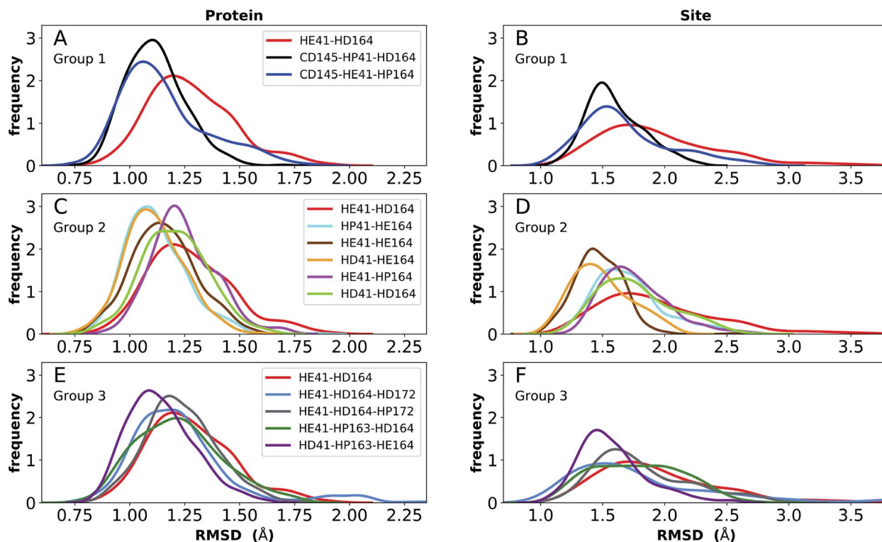
Fig. 3 RMSD distributions for the three protonation-state groups from simulations of the apo structure (PDB entry 6WQF † ). (A and B) RMSD of (A) protein and (B) active site for Group 1. (C and D) RMSD of (C) protein and (D) active site for Group 2. (E and F) RMSD of (E) protein and (F) active site for Group 3.
