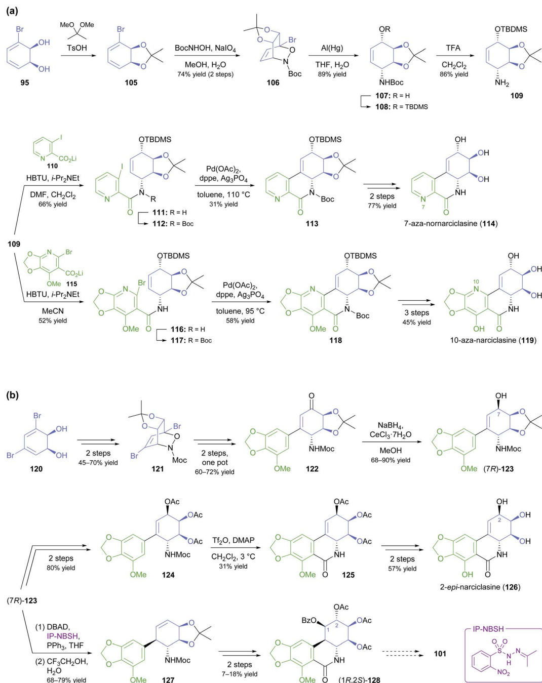
Scheme 16 Recent application of TDO-derived chiral building blocks in the synthesis of isocabostyryl alkaloids: (a) transformation of building block 95 into 7-aza-nornarciclasine (114) and 10-aza-narciclasine (119), (b) transformation of building block 120 into 2-epi-narciclasine (126) and a late synthetic intermediate 128 of (+)-pancratistatin (101).
