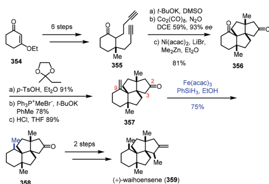
Scheme 44 Yang's synthesis of waihoensene (359).
