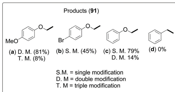
Scheme 23 Thiostrepton functionalization by Roelfes et al. 81
