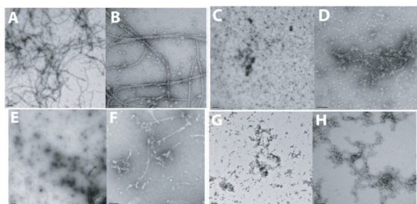
Fig. 2 N -Removable protecting groups in amyloid synthesis. Photolabile ( o -nitrobenzyl)glycine units are used in key peptide positions. (A and B) Transmission electron microscopy (TEM) of non-protected A \beta 1–42 at 24 h showed formation of long fibrils. (C and D) TEM at 24 h of A \beta 1–42 with backbone modification at Gly29 using the 2-nitrobenzyl group (NB). The introduction of NB inhibited fibril generation, but smaller oligomer aggregation could be observed. (E and F) TEM at 24 h of A \beta 1–42 with protecting groups in Gly29, Gly33 and Gly38. The hydrophobicity increased and also the aggregation of oligomers. (G and H) In A \beta 1–42 modified at Gly33 and Gly38, fibrils formed but were shorter and thinner than those in the native A \beta 1–42 sequence. TEM photos are originals from Meredith et al. , reproduced by license of Wiley-VCH. 113
