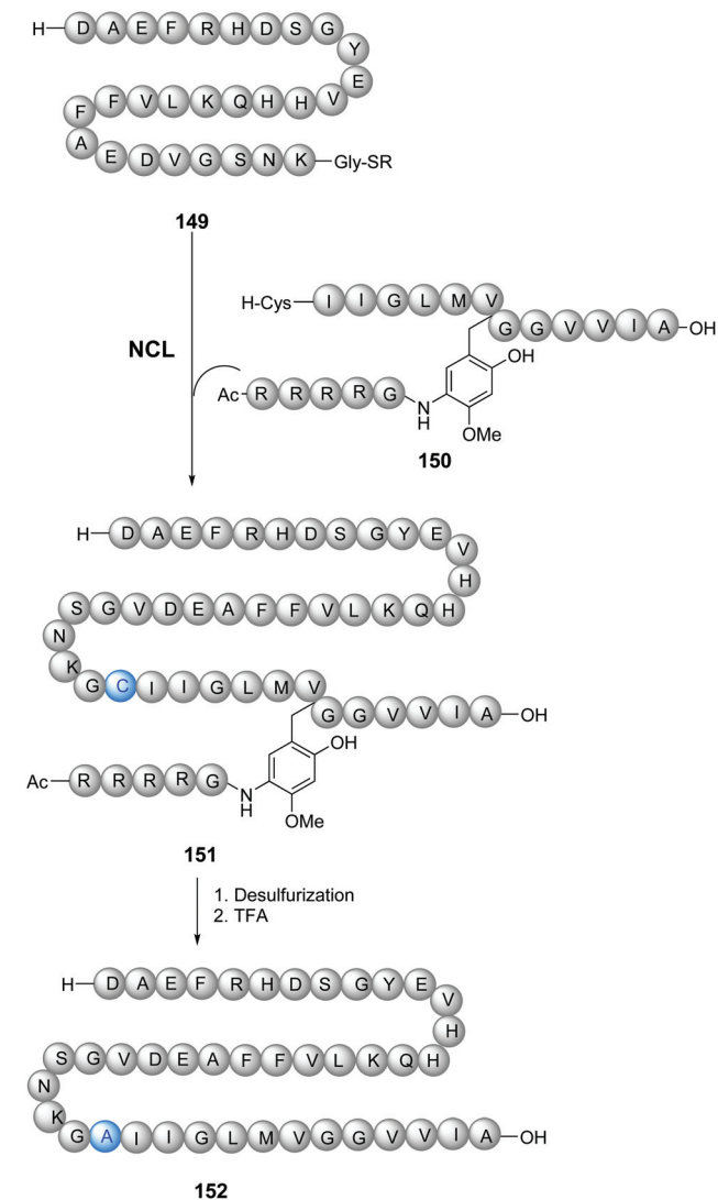
Scheme 36 N -Removable protecting groups to avoid aggregation in the synthesis of amyloid beta-peptides by Zheng et al. 115
