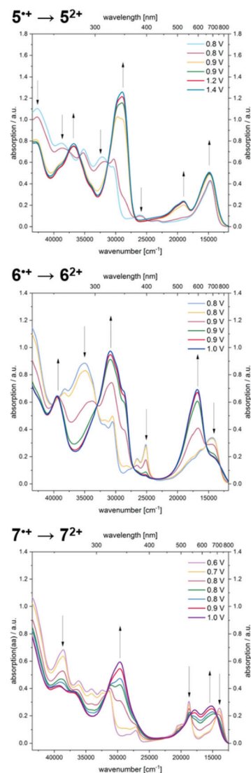
Fig. 8 UV/Vis spectroelectrochemical measurements of radical cations 5^{+} , 6^{+} , and 7^{+} forming the corresponding dicationic species 5^{2+} , 6^{2+} , and 7^{2+} ( \text{CH}_2\text{Cl}_2 , T = 293 K; electrolyte 0.1 M [\text{tBu}_4\text{N}][\text{PF}_6] ; Pt working electrode, Pt counter electrode and Ag/AgCl pseudo reference electrode).
