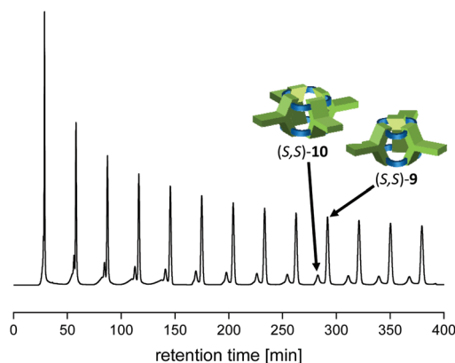
Fig. 2 Recycling-GPC chromatogram of the reaction of 7 with ( S,S )-8. For experimental details, see ESI†. Please note that in between the peak at 150 min and 160 min, the compounds responsible for the broad peak were removed.
