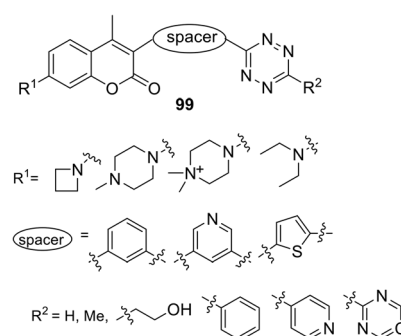
Fig. 17 Chemical structure of conjugates 99 .
