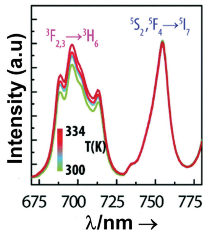
Fig. 10 Temperature dependence of the emission spectra of Ho,Tm:KLu(WO 4 ) 2 nanocrystals, demonstrating the similar intensity between the {}^3\text{F}_{2,3} \rightarrow {}^3\text{H}_6 of \text{Tm}^{3+} and {}^5\text{S}_2, {}^5\text{F}_4 \rightarrow {}^5\text{I}_7 of \text{Ho}^{3+} . Reprinted with permission from ref. 150. Copyright 2018, The Royal Society of Chemistry.
