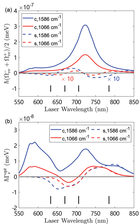
Fig. 5 (a) Vibrational frequency shift (\Omega_{\text{w}}^+ + \Omega_{\text{w}}^-)/2 and (b) effective optomechanical damping rate \Gamma_{\text{v}}^{\text{opt}} = \Gamma_{\text{w}}^- - \Gamma_{\text{w}}^+ as a function of the laser wavelength for the 1586 \text{cm}^{-1} vibrational mode (blue lines) and the 1066 \text{cm}^{-1} vibrational mode (red lines). The solid and dashed lines are the results from the continuum-field model (labeled as “c”) and the single-mode model (labeled as “s”), respectively. The vertical lines indicate wavelengths at 633 nm, 670 nm, 705.9 nm and 785 nm used for later simulations. The laser intensity is 1 \mu\text{W } \mu\text{m}^{-2} and other parameters are specified in the text.
