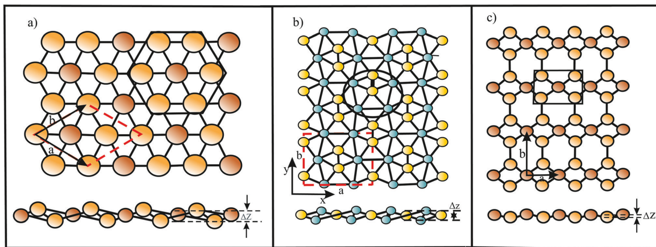
Fig. 9 (a) Top and side view of the Be 2 C monolayer. The black hexagon shows the quasi-phC motif and the red dashed rhombus displays the unit cell. Braun and yellow balls represent C and Be atoms, respectively, a and b are the lattice vectors, and \Delta z is the buckling effect. (b) Top and side view of the CaSi monolayer, containing the quasi-ppSi motif as indicated by the black circle. The yellow and blue balls present the Si and Ca atoms, respectively. The red dashed lines label the unit cell. (c) Top and side view of the B 2 C monolayer with quasi-ptC motif. Braun and yellow balls are the C and B atoms, respectively. The black rectangular box shows the quasi-ptC motif.
