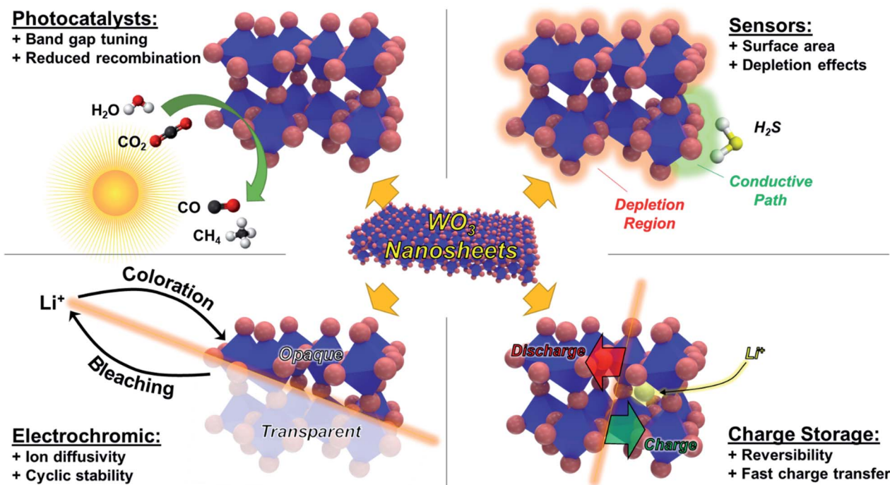
Fig. 1 Schematic showing basic principles of operation for WO 3 in photocatalysts, sensors, electrochromic devices, and charge storage applications, along with the potential advantages provided by the nanosheet morphology.
