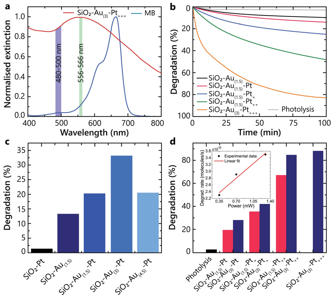
Fig. 3 The effect of Au and Pt loading. (a) Normalised optical extinction of MB and the \text{SiO}_2\text{-Au}_{(3)}\text{-Pt}_{+++} heterostructures measured in water. (b) Time evolution of the MB absorbance during the illumination for hetero-nanoparticles with different Pt loading. (c and d) Photocatalytic degradation dependence on (c) Au and (d) Pt loading. For photodegradation, the pulsed laser illumination was used in a 556–566 nm spectral range with an average power of 0.35 mW. Inset in (d) shows the initial degradation rate dependence on the illuminating power for \text{SiO}_2\text{-Au}_{(3)}\text{-Pt} nanoparticles.
