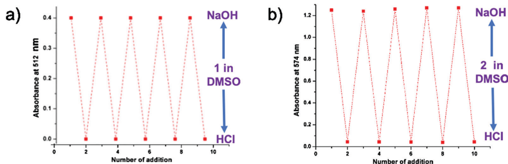
Fig. 6 Reversible changes in the UV-absorption of DMSO solution of (a) probe 1 at 512 nm and (b) probe 2 at 574 nm.
