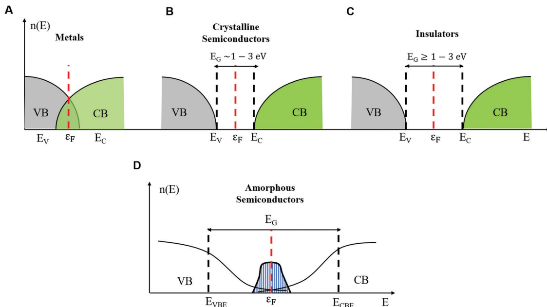
Fig. 1 Density of electronic states in the energy landscape showing the band gap and the Fermi level for (A) metals, (B) crystalline semiconductors, (C) insulators and (D) amorphous semiconductors.
