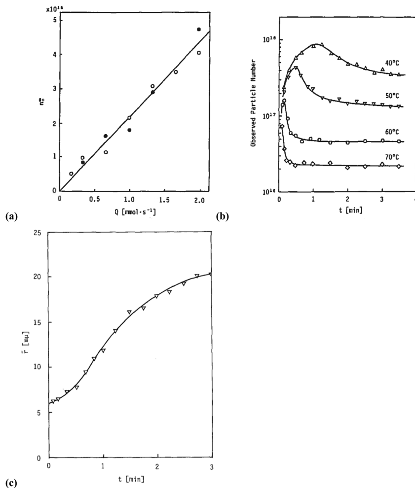
Fig. 6 (Fig. 9, 11 and 15 in ref. 100.) (a) The final number of observed particles ( n_p^+ ) as a function of Q , “the molal feed rate of the monomer source into the system”, 100 at 70 °C and pBr 3.0 in the (\text{AgBr})_n formation open system. The closed circles represent a repeat set of experiments at the same Q values. (b) The number of the observed particles ( n_p^+ ) as a function of time at different temperature ( Q = 10^{-3} \text{ mol s}^{-1} and pBr 3.0). (c) The change of the mean radius, \bar{r} , of “nuclei” (in the author’s 100 nomenclature; really the growing particle) as a function of time in the early stage of precipitations at 50 °C. Observed lines are arbitrary and do not represent any fitting function. Reproduced with permission from ref. 100. Copyright 1992 Academic Press, Inc.
