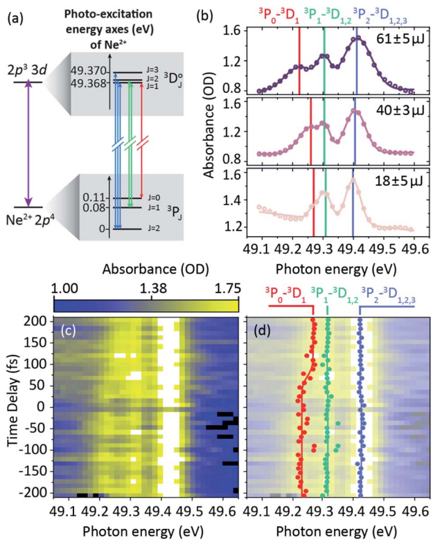
Fig. 7 (a) Level scheme of the resonant coupling mechanism of the \text{Ne}^{2+} ion. Observed absorption lines correspond to the ground-state splitting, while the 1 meV-scale excited-state splitting is unresolved. The observed sets of multiplet transitions are indicated in blue, green, and red. (b) Static absorption spectroscopy of the pump pulse evaluated at large negative delays (probe first) for the mean pulse energies 18 \pm 5 \mu\text{J} (pulse-energy range <25 \mu\text{J} ), 40 \pm 3 \mu\text{J} (pulse-energy range 35\text{--}45 \mu\text{J} ), and 61 \pm 5 \mu\text{J} (pulse-energy range >55 \mu\text{J} ). Also see ref. 3 for further details on the experiment. (c) Time-resolved absorption data of the pump pulse at 69 \pm 3 \mu\text{J} mean pulse energy (pulse-energy range indicated in dark violet in Fig. 5b). (d) Fitted spectral positions of the observed lines (data points) and error-function fit to the fit results over time delay (corresponding solid lines) to find temporal duration and position of the transient spectral shift.
