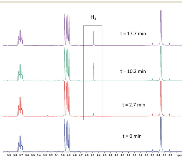
Fig. 8 ^1\text{H} NMR spectra showing the appearance of dissolved \text{H}_2 during [\text{Rh}(\text{CO})_2(\text{acac})] + 6\text{PPh}_3 catalysed hydroformylation of 1-hexene in toluene at 50 °C and 12 bar of \text{H}_2/\text{CO} (1 : 1) from operando ^1\text{H} FlowNMR spectroscopy. [\text{Rh}(\text{CO})_2(\text{acac})] = 2.5 \text{ mM} , [\text{PPh}_3] = 15 \text{ mM} , [1\text{-hexene}] = 500 \text{ mM} .
