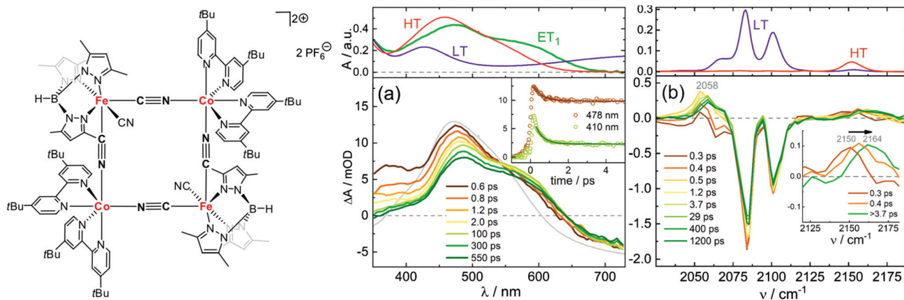
Fig. 2 Structure of [(\text{Co}_{\text{LS}}^{\text{II}})_2(\text{Fe}_{\text{LS}}^{\text{II}})_2] together with transient absorption data in acetonitrile at -30\text{ }^\circ\text{C} with (a) UV-visible probe and 775 nm pump wavelength and (b) IR probe and 800 nm pump. The top panels show the static absorption spectra in the LT ( -30\text{ }^\circ\text{C} ) and HT ( 30\text{ }^\circ\text{C} ) phases. The green line (ET1) corresponds to the calculated spectrum of the one-electron transfer product [\text{Co}_{\text{LS}}^{\text{III}}\text{Fe}_{\text{LS}}^{\text{II}}\text{Co}_{\text{HS}}^{\text{II}}\text{Fe}_{\text{LS}}^{\text{II}}] . The bottom panels show the time-resolved spectra at selected time delays. The grey line shows the difference between the HT and LT static spectra. Reprinted with permission from Zimara et al. Inorganic Chemistry , 2021, 60 , 449–459. 116 Copyright 2021 American Chemical Society.
