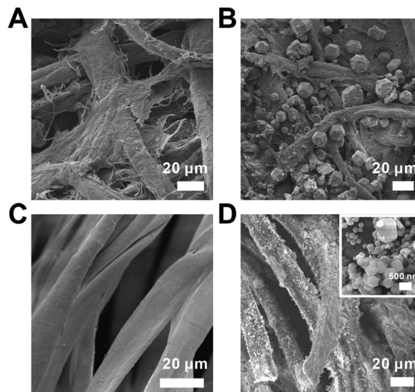
Fig. 2 SEM images of the (A) filter paper, (B) ZIF-8 on filter, (C) cotton fabric, and (D) ZIF-8 on cotton (the inset is a close-up image of the ZIF-8 particle on the fibre surface).
