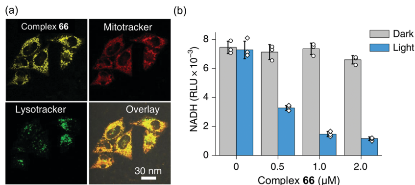
Fig. 18 (a) Confocal microscopy images showing mitochondrial localization of the photosensitizer complex 66 . (b) NADH concentration in A549 cells treated with complex 66 with or without photo-irradiation. Reproduced from ref. 51 with permission.
