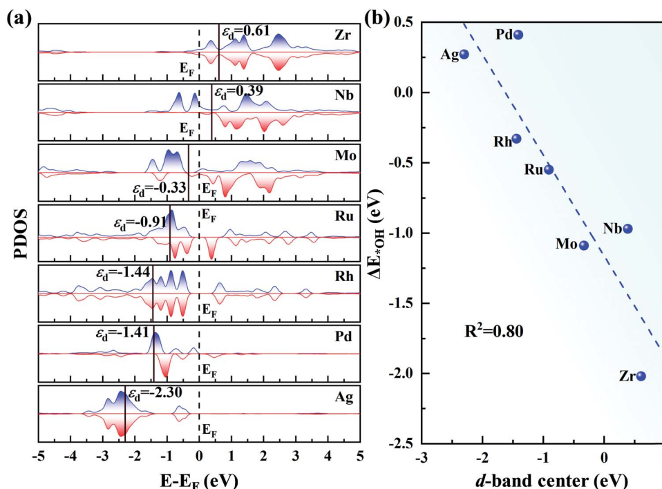
Fig. 7 (a) Partial density of states of the 4d TM atoms on g- \text{C}_3\text{N}_4 , where E_{\text{F}} denotes the Fermi level and is set to zero. (b) Relationship between the d-band centre of TM/g- \text{C}_3\text{N}_4 and \Delta E_{*_{\text{OH}}} .
