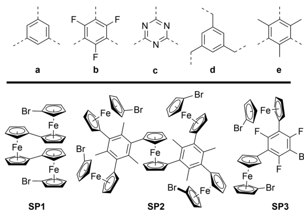
Scheme 1 (Top) Preparation of tris-phosphanes 1a–d and complexes [(1a–c)E] . (I) Pd precatalyst, THF, r. t.; (II) n BuLi, Ph 2 PCL, THF, –80 °C to r. t.; (III) [E]·X ([E]·X = BH 3 ·SMe 2 or [AuCl(ths)], CH 2 Cl 2 , r. t.; (Bottom) crystallographically characterised side products obtained during the syntheses of 4d (SP1), 4e (SP2), and 4b (SP3). For their solid-state structures, see Fig. S3.†
