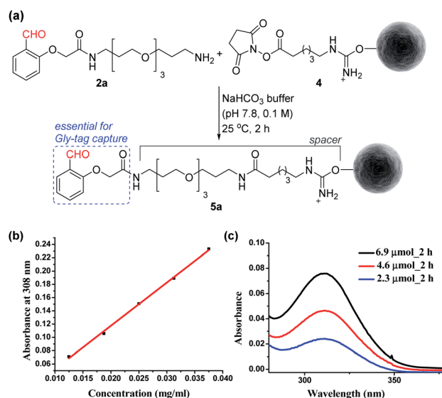
Fig. 3 (a) Synthesis of the Gly-tag purification resin. (b) Determination of the molar extinction coefficient of the reagent 2a. (c) Estimation of unbound reagent 2a by UV absorption after reaction with resin 4 (2.3 μmol).
