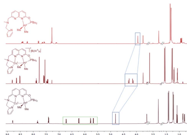
Fig. 2 1 H NMR spectra (THF- d 8 , 25 °C) of isolated complexes 1 (top), 3 [B(Ar F ) 4 ] (middle) and dearomatized complex 4 (bottom). Blue rectangles highlight the naphthyridine-CH 2 signal or CH for 4 . Green rectangle highlights the naphthyridine C sp 2 -H signals of 4 .
