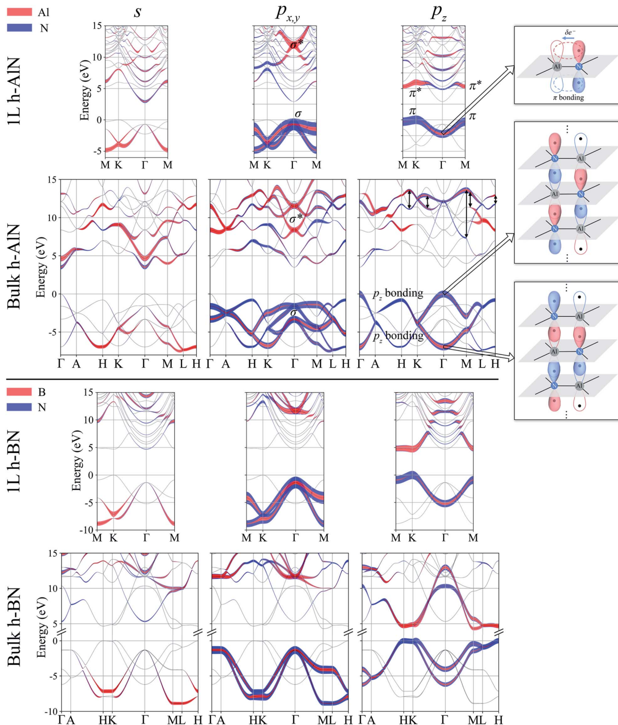
Fig. 6 Fat band plots showing projected weights onto cation- and anion-centered s , p_{x,y} , and p_z orbitals for 1L and bulk h-AIN (upper panel), compared with those of h-BN (lower panel). For h-AIN, band states with predominant \sigma , \sigma^* and \pi , \pi^* characters are labeled in the p_{x,y} and p_z plots, respectively. Going from 1L to bulk, the \pi band splits into two p_z bonding bands, and the \pi^* band can be largely considered to split into two p_z antibonding bands as indicated by the double headed arrows; the p_z antibonding bands exhibit considerable mixing with \sigma^* and free-electron-like bands. Bonding schemes derived from the projection are visualized on the right, where the \sigma bonds are depicted as thick black lines and the p_z orbitals as balloons with colors (red and blue) signifying orbital wavefunction signs, solid filling indicating filled orbitals, and each dot visualizing an electron.
