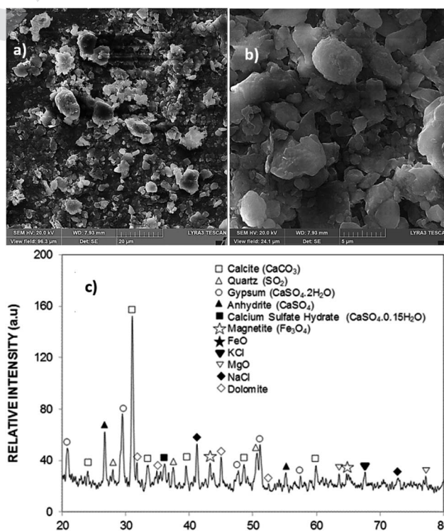
Fig. 1 The SEM micrographs and the X-ray diffractogram of dust: (a) the SEM micrograph of dust particles with various shapes and sizes, (b) the clustered dust particles, and (c) the X-ray diffractogram of dust.
