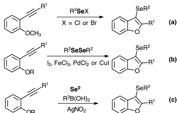
Scheme 1 Methodologies to prepare 3-selanyl-benzo[ b ]furans.
