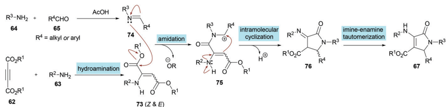
Scheme 17 Proposed mechanism for the formation of polysubstituted dihydropyrroles 67 .
