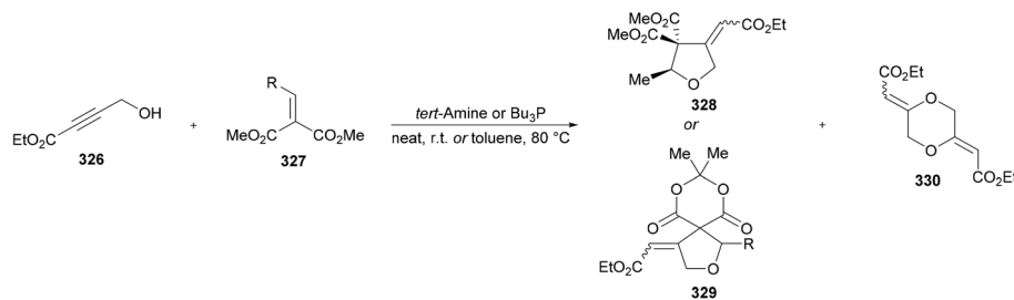
Scheme 82 Phosphine-catalyzed synthesis of functionalized tetrahydrofurans using electron-deficient propargyl alcohols and Michael acceptors.
