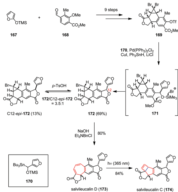
Scheme 24 4π electrocyclization in the total synthesis of salvileucalin C.
