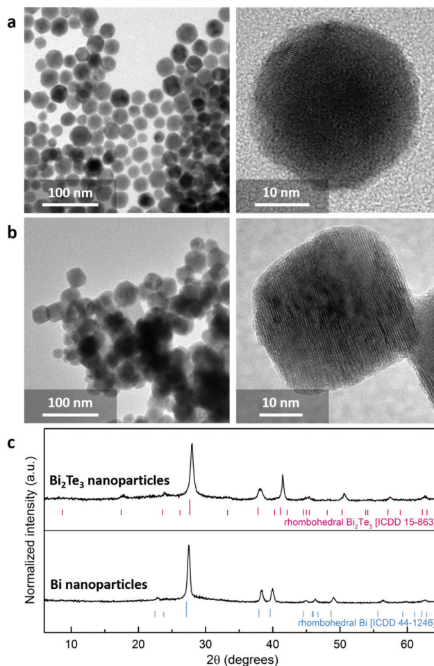
Fig. 2 \text{Bi}_2\text{Te}_3 nanoparticle synthesis: (a) TEM images of Bi nanoparticles, which are nearly spherical and of average radius 14.4 nm. (b) Successfully synthesized \text{Bi}_2\text{Te}_3 nanoparticles with a slightly rhombohedral shape and average radius of 17.5 nm. (c) X-ray diffraction patterns illustrating the successful tellurisation of the Bi nanoparticles to form \text{Bi}_2\text{Te}_3 nanoparticles.
