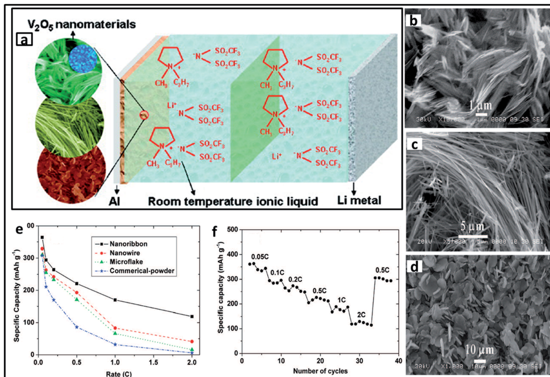
Fig. 15 (a) Schematic representation of a lithium metal battery using \text{V}_2\text{O}_5 nanomaterials and room temperature ionic liquid electrolyte. SEM images of diverse morphologies of \text{V}_2\text{O}_5 materials: (b) nanoribbons (c) nanowires (d) microflakes and their corresponding (e) specific capacities; (f) cycle life of \text{V}_2\text{O}_5 nanoribbon. "Adapted with permission from ref. 218. Copyright (2008) American Chemical Society."
