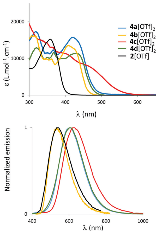
Fig. 3 UV-Vis absorption (top) and normalized emission spectra (bottom) of 2[\text{OTf}] and 4\mathbf{ad}[\text{OTf}]_2 in \text{CH}_2\text{Cl}_2 ( c = 5 \times 10^{-6} \text{ M} ).
