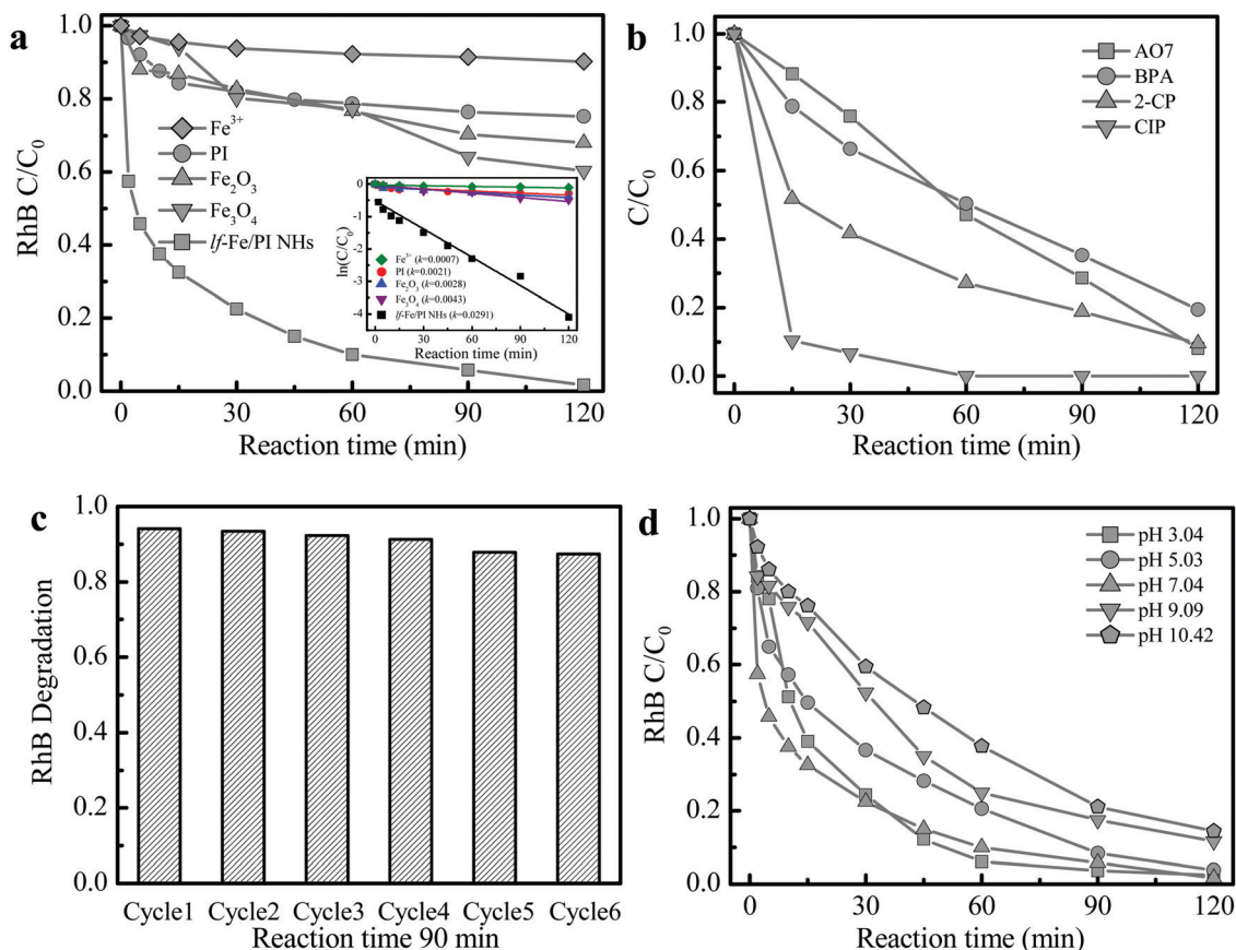
Fig. 5 Performance of lf-Fe/PI HNs for pollutant removal. (a) RhB degradation curves in various suspensions with H_2O_2 (inset shows the corresponding kinetic curves). (b) Decomposition curves of other different pollutants in the lf-Fe/PI HNs suspensions with H_2O_2 . (c) Reusability of lf-Fe/PI HNs for RhB degradation. (d) Effect of initial pH values for RhB degradation. Reaction conditions: natural initial pH (pH 6–7, except (d)), initial pollutants 10 \text{ mg L}^{-1} , initial H_2O_2 10 \text{ mM} , catalyst 1.0 \text{ g L}^{-1} (Fe ions 0.15 \text{ mg L}^{-1} in (a)).
