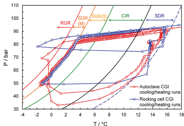
Fig. 18 Experimentally identified crystal growth inhibition (CGI) regions for 0.5 wt% PVCap in aqueous phase + methane; SDR: slow dissociation region, CIR: complete inhibition region, SGR(S), slow growth region (slow), SGR(M), slow growth region (medium), and RGR: rapid growth region. CGI cooling and heating tests for 0.5 wt% PVCap in aqueous phase + methane in the rocking cell and standard autoclave setups (adapted with permission from Mozaffar et al. , 1135 Copyright 2016 American Chemical Society).
