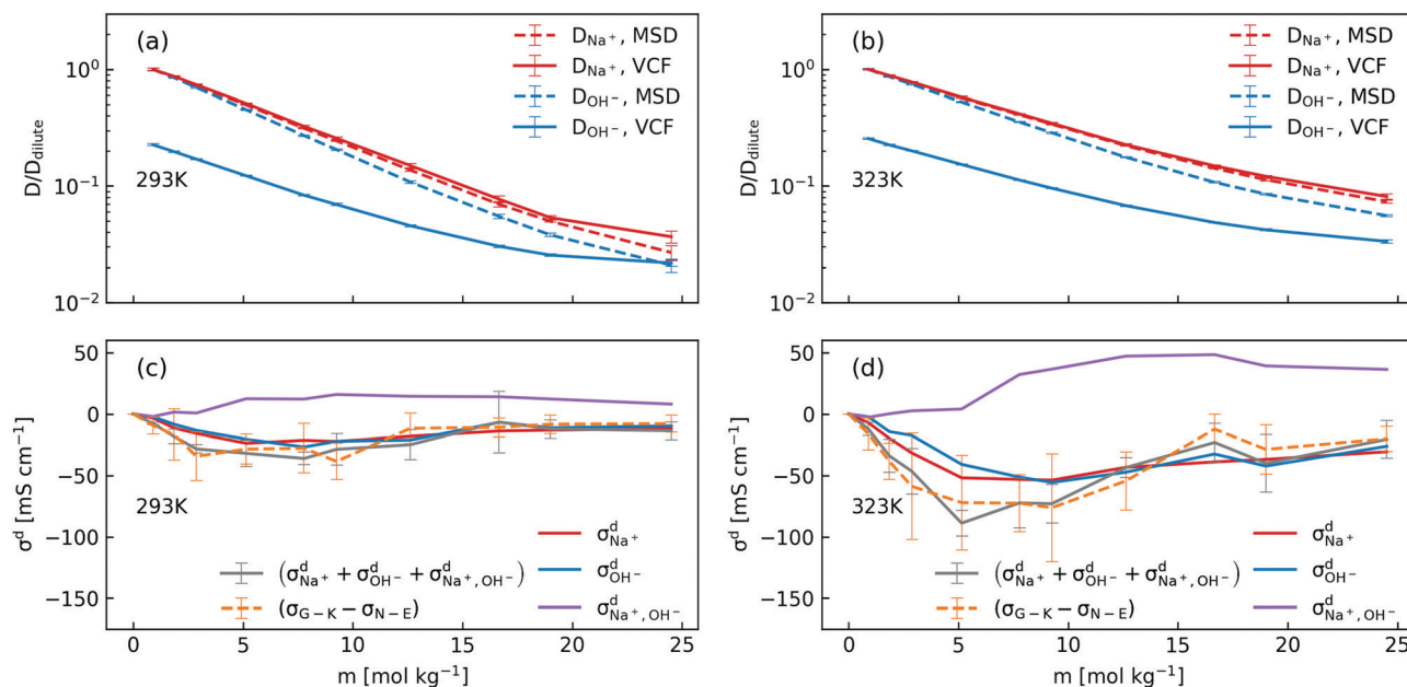
Fig. 2 (a) and (b) Scaled concentration-dependent self-diffusion coefficients of Na ^{+} and OH ^{-} at 293 K and 323 K obtained from VCF (eqn (2)) and from MSD (eqn (3)), where the self-diffusion coefficients were scaled by the corresponding value in the dilute solution; (c) and (d) contributions of distinct diffusion coefficients to the ionic conductivity at 293 K and 323 K as shown in eqn (7) and calculated from VCFs. Detailed definition of distinct diffusion coefficients can be found in ref. 28 and 32. Note that (\sigma_{\text{G-K}} - \sigma_{\text{N-E}}) were obtained from Fig. 1a for the purpose of comparison.
