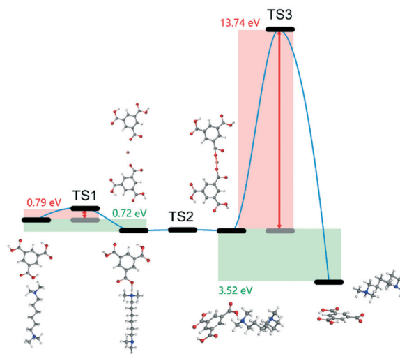
Fig. 6 Minimum energy path for hierarchically porous MOF synthesis with the corresponding intermediates and transition states, calculated at the GGA-PBE level.
