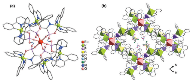
Fig. 13 (a) The heptanuclear cluster of 58 . (b) Packing diagram of 58 viewed along the c -axis. Color codes: \text{EuO}_6 , red; \text{IrC}_2\text{N}_3\text{O} , yellow green; \text{PO}_3\text{C} , purple. Adapted from ref. 65.
