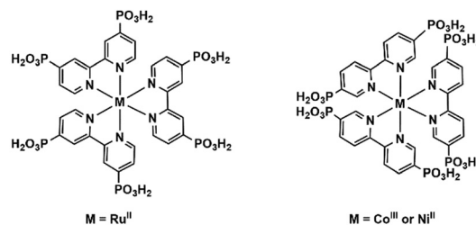
Scheme 8 Molecular structures of metalloligands \text{Ru}^{\text{II}}(4,4'\text{-dpbpyH}_4)_3^{2+} and [\text{M}(5,5'\text{-dpbpyH}_4)_3]^{n+} .
