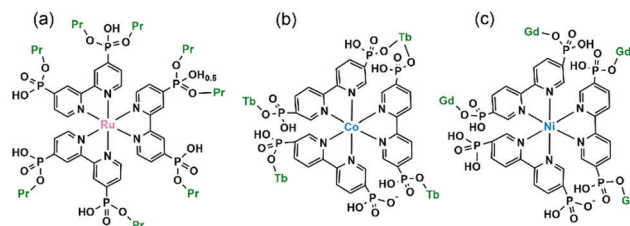
Scheme 9 Coordination modes of metalloligands \text{Ru}^{\text{II}}(4,4'\text{-dpbpyH}_4)_3^{2+} and [\text{M}(5,5'\text{-dpbpyH}_4)_3]^{n+} .
