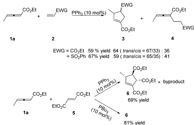
Scheme 2 Phosphine-catalysed (3+2) cycloaddition reactions of acrylate, vinyl phenyl sulfone or fumarate with \gamma -methyl allenate.
