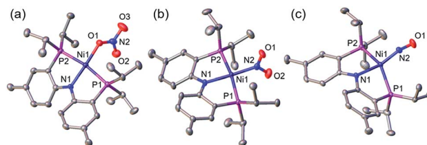
Fig. 3 Displacement ellipsoid (50%) representation of (a) (PNP)Ni(ONO_2) ( 1 ), (b) (PNP)Ni(NO_2) ( 2 ) and (c) (PNP)Ni(NO) ( 3 ). Hydrogen atoms and molecules of cocrystallization are omitted for clarity.
