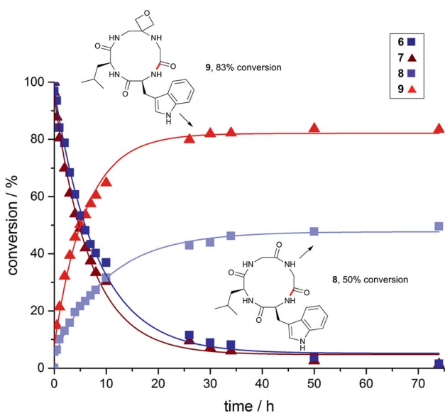
Fig. 2 Impact of oxetane modification on macrocyclisation rates: Cyclisation of WLGG ( 6 ) and oxetane modified WLGOxG ( 7 ) monitored over 74 h using DEPBT (2 equiv.), 1 Pr 2 EtN (2 equiv.) in DMF (0.001 M), RT. Bond formed in macrocyclisation indicated in red; peptides were quantified by analytical HPLC by integration of the corresponding UV signal at 280 nm (see ESI†).
