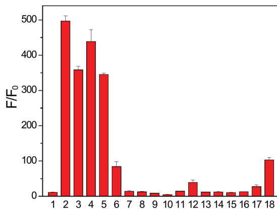
Fig. 5 Fluorescence turn on of FLD-1 (10 \mu M) in the presence of cellular RSONs (100 \mu M): (1) FLD-1 only, (2) Cys, (3) NAC, (4) GSH, (5) Hcy, (6) PEN, (7) BSA, (8) Cys + NEM, (9) H 2 O 2 , (10) ClO - , (11) O 2 - , (12) TBHP, (13) Ser, (14) Lys, (15) Gly, (16) GSSG, (17) GSNO, and (18) PLE (1 U mL -1 ). Fluorescence intensity was measured after 2 h incubation. The experiments were performed in triplicate. The results were expressed as mean \pm SD ( n = 3 ).
