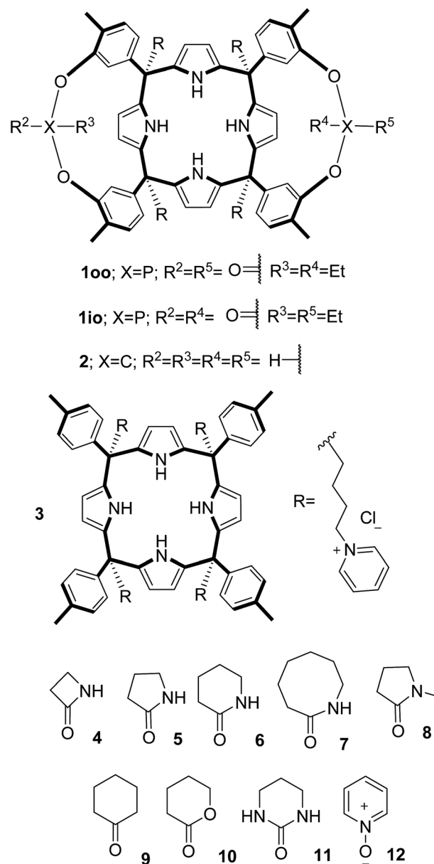
Fig. 3 Molecular structures of the four water-soluble aryl-extended calix[4]pyrrole derivatives, 1oo , 1io , 2 and 3 , and of the guests, 4 – 12 , used in this study.
