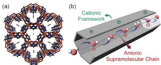
Fig. 11 (a) Crystal structure of [\text{Ni}_2(m\text{-pymca})_3]\text{OH}\cdot n\text{H}_2\text{O} along the channel. (b) Schematic representation of a cationic MOF with an anionic supramolecular chain of hydroxide anions and water molecules inside the MOF pore for efficient hydroxide ion conduction. Reproduced from ref. 55 with permission from Royal Society of Chemistry, Copyright 2016.
