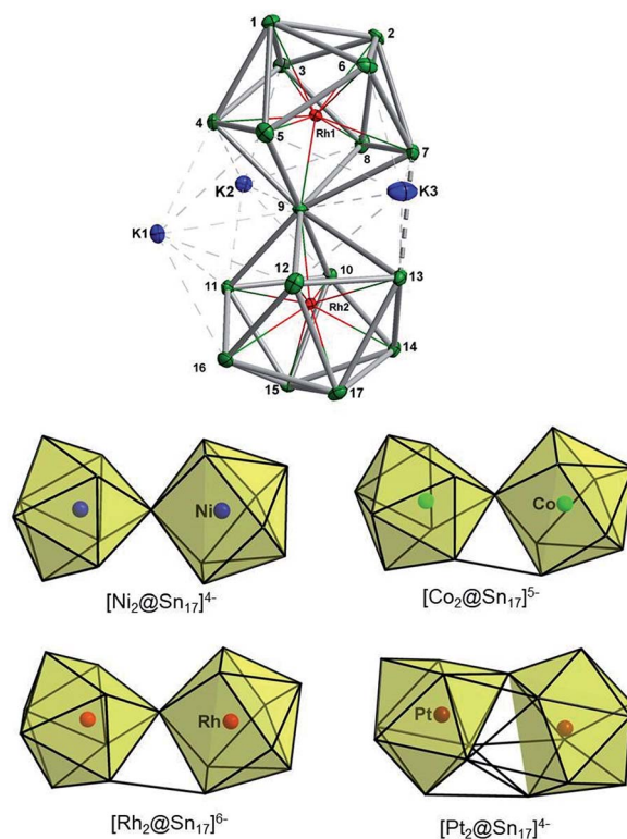
Fig. 4 Top: Thermal ellipsoid plots of the [\text{Rh}_2@ \text{Sn}_{17}]^{6-} anion and its three tightly bound \text{K}^+ cations (drawn at 50% probability). Bottom: Comparison of the known structures of M_2@ \text{Sn}_{17} anions, M = \text{Ni} , 18a \text{Co} , 5b \text{Rh} and \text{Pt} . 18b
