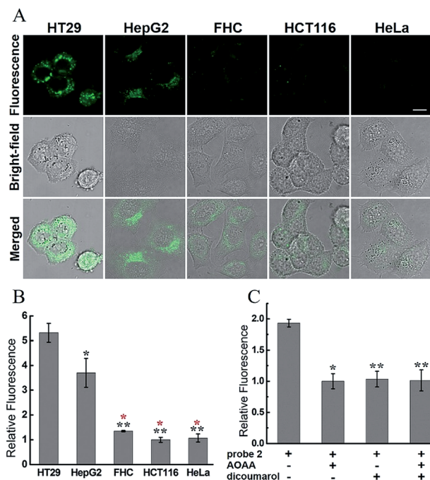
Fig. 6 Confocal microscopy images for endogenous H_2S and hNQO1 detection in living cells using 2. (A) Cells ( \sim 2 \times 10^4 cells per well) were incubated with only 2 (10 \mu M ) for 1 h, washed, then imaged. Scale bar, 10 \mu m . (B) Relative fluorescence intensity of images from (A). (C) Relative fluorescence intensity of images from inhibitor-pretreated HT29 cells. N = 3 fields of cells, error bars are means \pm sd. * P < 0.05 ; ** P < 0.01 . For (B), the black * was relative to HT29 group, and the red * was relative to HepG2 group.
