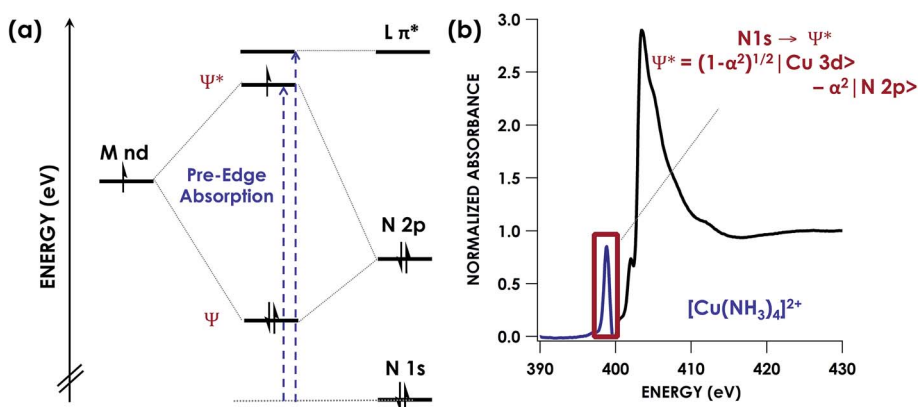
Fig. 1 (a) Simplified energy level diagram showing representative orbitals involved during pre-edge excitations in N K-edge XAS. (b) Representative N K-edge XAS spectrum of [Cu(NH 3 ) 4 ]SO 4 with computationally validated pre-edge band assignment.
